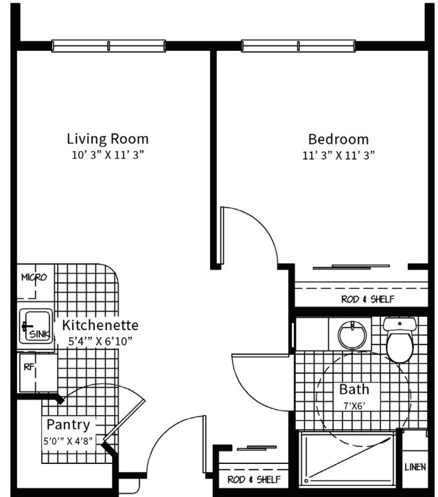
One Bedroom 572 Square Feet
